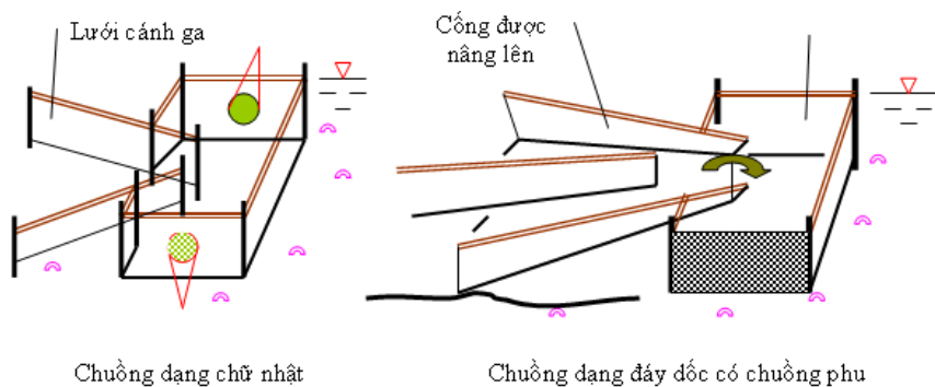
Set net
