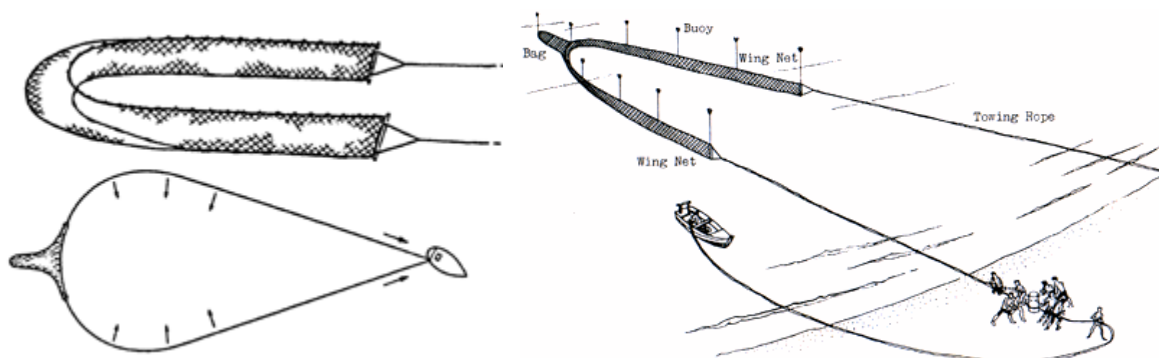
Beach Seine (top) and Boat seine (bottom)
